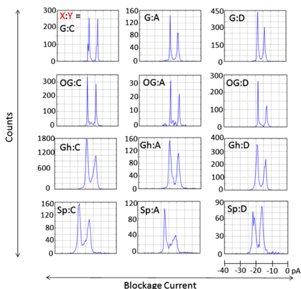
Figure 3. Histograms of the blockage current for the duplex formed by hybridizing the X-containing 65-mer with the Y-containing 17-mer at -120 mV. X:Y represents the modified base pair.
