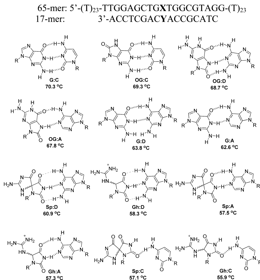
Figure 1. Base-pairing schemes for X:Y (X = G, OG, Sp, or Gh and Y = C, A, or D). The base pairs G:A, G:C, OG:A, and OG:C are drawn on the basis of reported structural data, whereas the hydantoin base pairs are drawn on the basis of predictions in refs 6 and 38. The duplexes are arranged in order of decreasing melting temperatures (from top down). The D-containing base pairs are predicted on the basis of their H-bonding capabilities as discussed in the text. The melting temperatures are listed under each X:Y-containing duplex and have an average standard deviation of 0.6 °C (see the Supporting Information for individual standard deviations in T_m ).
