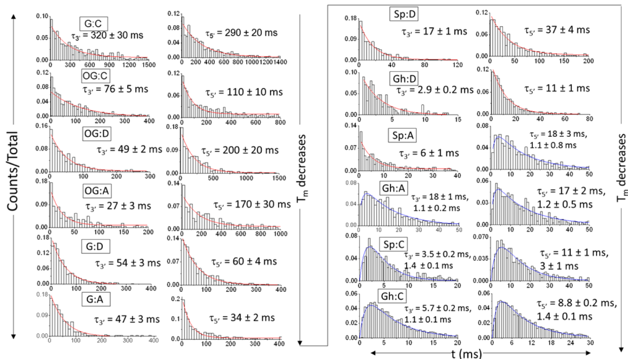
Figure 4. Histograms of unzipping time ( t ) via 3' entry (left column) and 5' entry (right column) at -120 mV for the duplex that contains X:Y (where X = G, OG, Gh or Sp and Y = C, A, D). The unzipping time constants ( \tau ) were obtained on the basis of the fit (red or blue curves) of the t histograms using the corresponding kinetic model, either a first-order reaction (Type I, red) or two sequential first-order reactions (Type II, blue). If the strand dissociation follows the Type II model, then the unzipping time constants for each step are presented without assignment of the first and second steps. The histograms are plotted on different time scales to emphasize the shape as a determinant for the model type.
