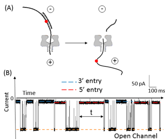
Figure 2. Unzipping of a DNA duplex using an \alpha -HL nanopore under an electrical field. (A) dsDNA strand dissociation within an \alpha -HL channel. The red dot in the target strand defines the relative position of X (X = G, OG, Sp, or Gh) opposite to Y (Y = C, A, or D) in the duplex. The + and - signs show the polarity of the electrodes. (B) Example of a current–time trace (X:Y = OG:C) at an applied voltage of -120 mV (cis versus trans). The blockades that last up to hundreds of milliseconds correspond to unzipping events of duplexes (unzipping duration shown as t ). Events with duration shorter than 0.5 ms correspond to translocation of excess 17-mer ssDNA (the 65-mer and 17-mer strands are present in a 1:5 mol ratio). The red and blue dashed lines show the current blockage levels associated with 5' and 3' entry, respectively.
